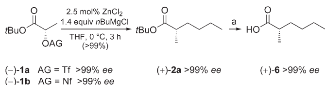
Scheme 2. Determination of the absolute configuration of 2a . a) TFA (trifluoroacetic acid), CH 2 Cl 2 , RT, > 99%. Tf = trifluoromethanesulfonyl, Nf = nonafluorobutanesulfonyl.
